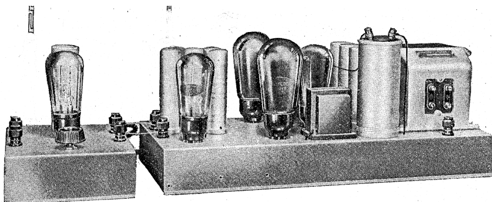
1934. The "Wireless World Quality Push Pull Amplifier" Push pull configuration main amplifier with driver pre-stage. Triode output, RC coupling, no feedback, 5-7 watts.
