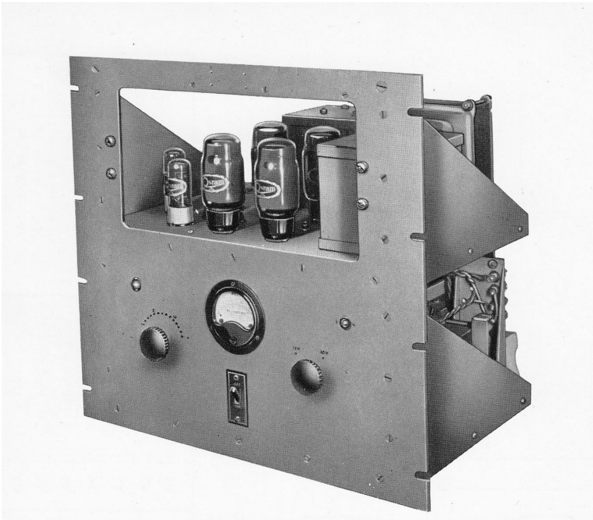
1945. An experimental 30 watt amplifier designed by D.T.N.Williamson for the Marconi Osram Valve Co. using four KT66 valves triode connected.
