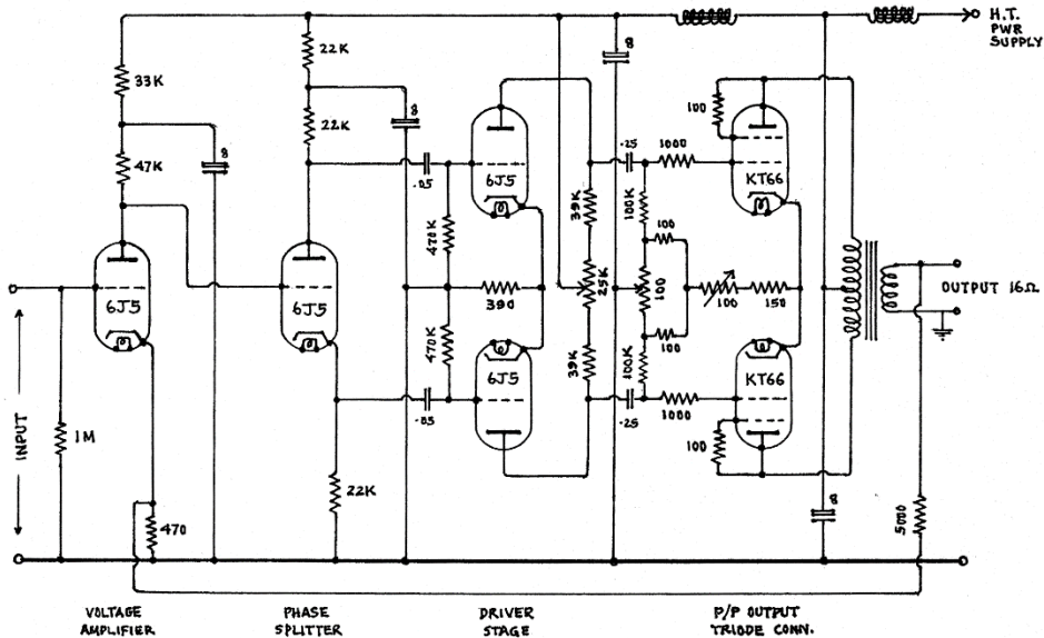
1947. The original circuit for Williamson’s amplifier as published by WIRELESS WORLD. Triode connected push pull KT66 output with 20dB feedback. An output transformer of the highest quality is an integral requirement of the design.
