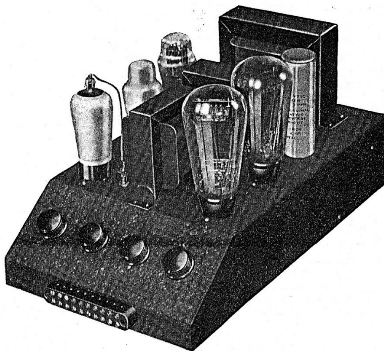
1938. A 12 watt amplifier by Partridge Transformers Ltd, England. Push pull triode output, transformer coupled, no feedback. A similar "Quality" unit was also available with an all triode circuit and higher grade transformers. Output transformer integral with the design.
