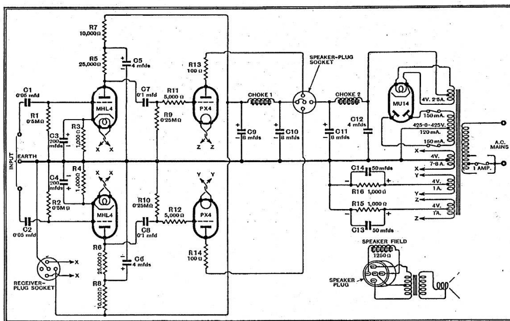
1934. The circuit for the Wireless World Quality Push Pull Amplifier. An additional pre-stage to provide the push pull drive was also described. Output transformer to be chosen by the user, according to the loudspeaker to be used.
