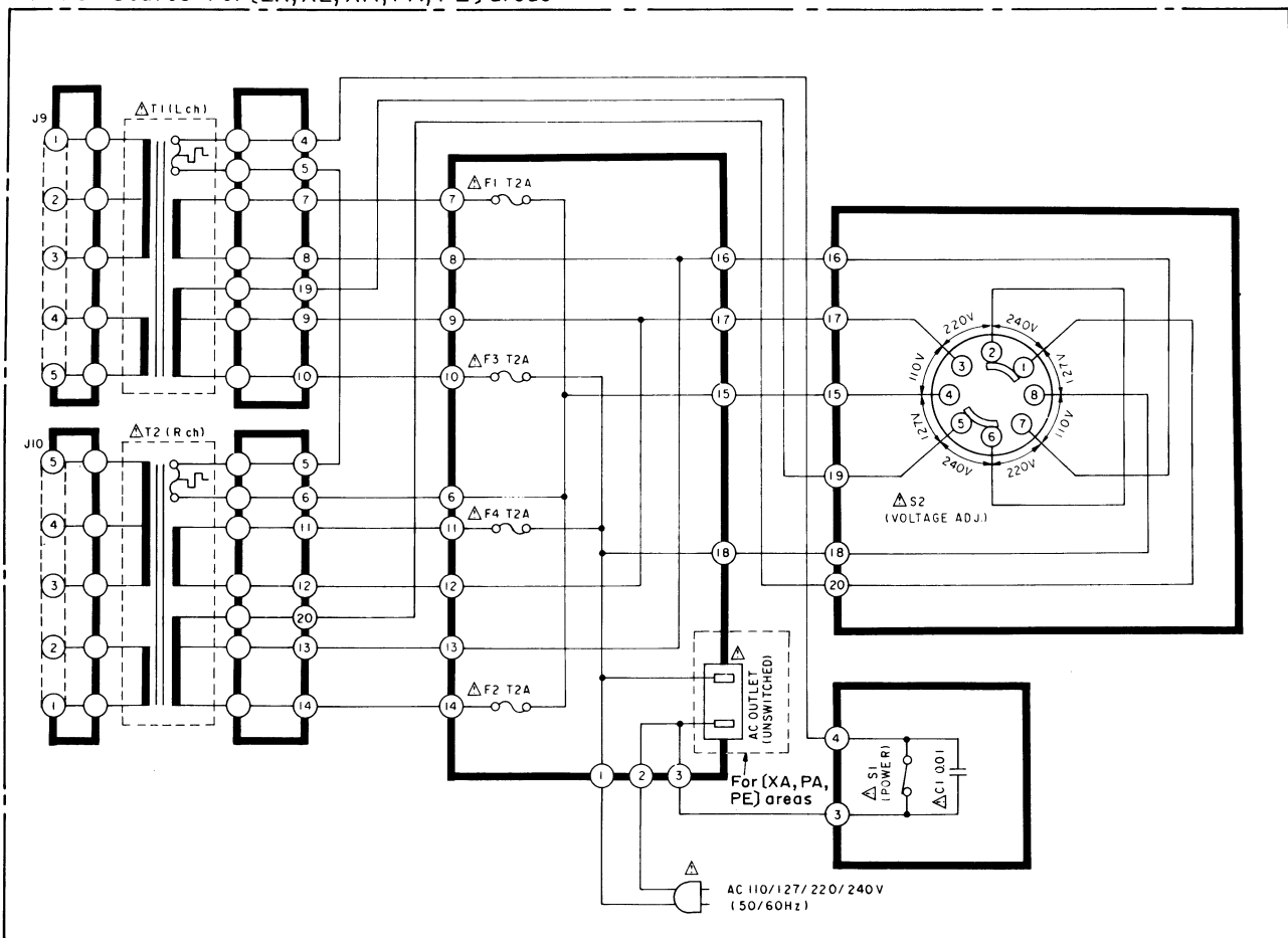
Power Source For [EK,XL,XA,PA,PE] areas
